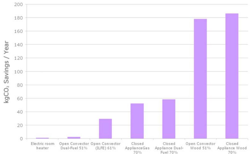
Graph 1. CO 2 variance for appliance, fuel and flue types
